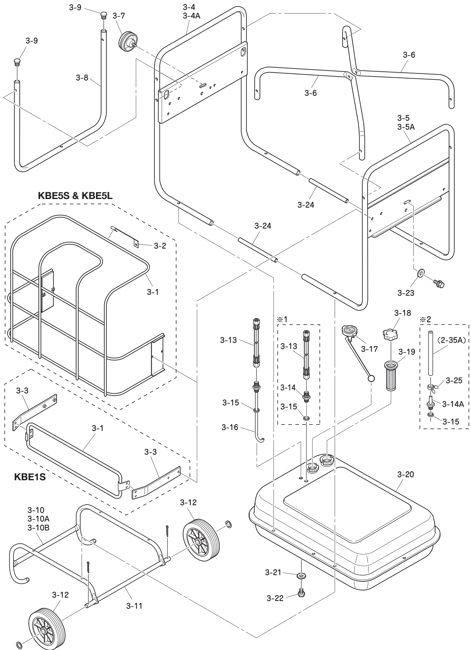
VAL6 KBE1S/5S/5L Tank Section_ Revised 2011
